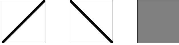
Figure 1: The limits of sequences (\pi_i^1)_{i \in \mathbb{N}} , (\pi_i^2)_{i \in \mathbb{N}} , (\pi_i^3)_{i \in \mathbb{N}} .
