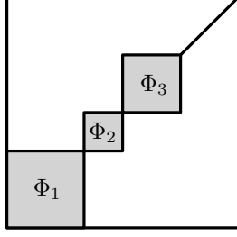
Figure 3: The permuton (1/3, \Phi_1) \oplus (1/6, \Phi_2) \oplus (1/4, \Phi_3) .
