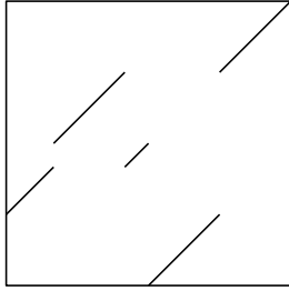
Figure 2: The permuton \Phi_\sigma^{\mathbf{v}} for \sigma = (2, 4, 3, 1) and \mathbf{v} = (1/6, 1/4, 1/12, 1/4) .
